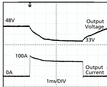
Peak load 100A (resistive) for 5ms Output voltage dips from 48V to 33V.
