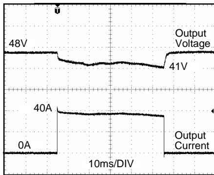
Peak load 40A (resistive) for 50ms Output voltage dips from 48V to 41V.
